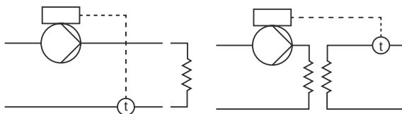
Fig. 46 Constant temperature
