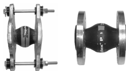
Fig. 82 Examples of rubber bellows expansion joints
